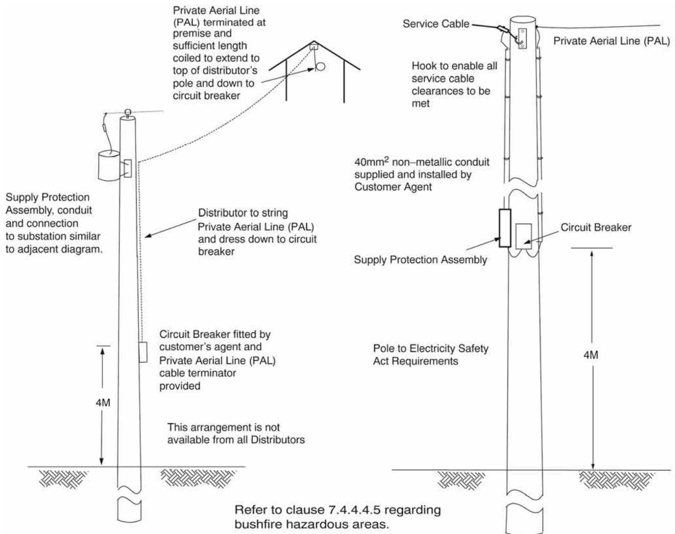
Figure 7.5-E Typical PAL Arrangements
