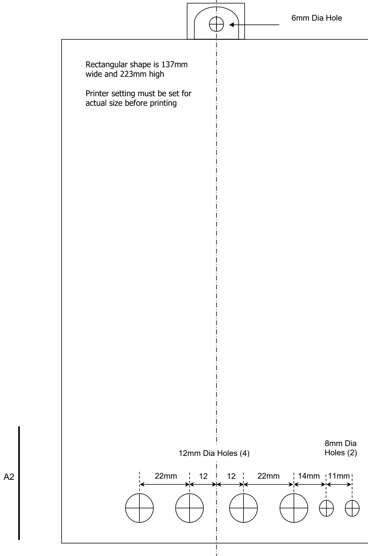
Figure 8.10-W Single Phase Meter Drilling Template
