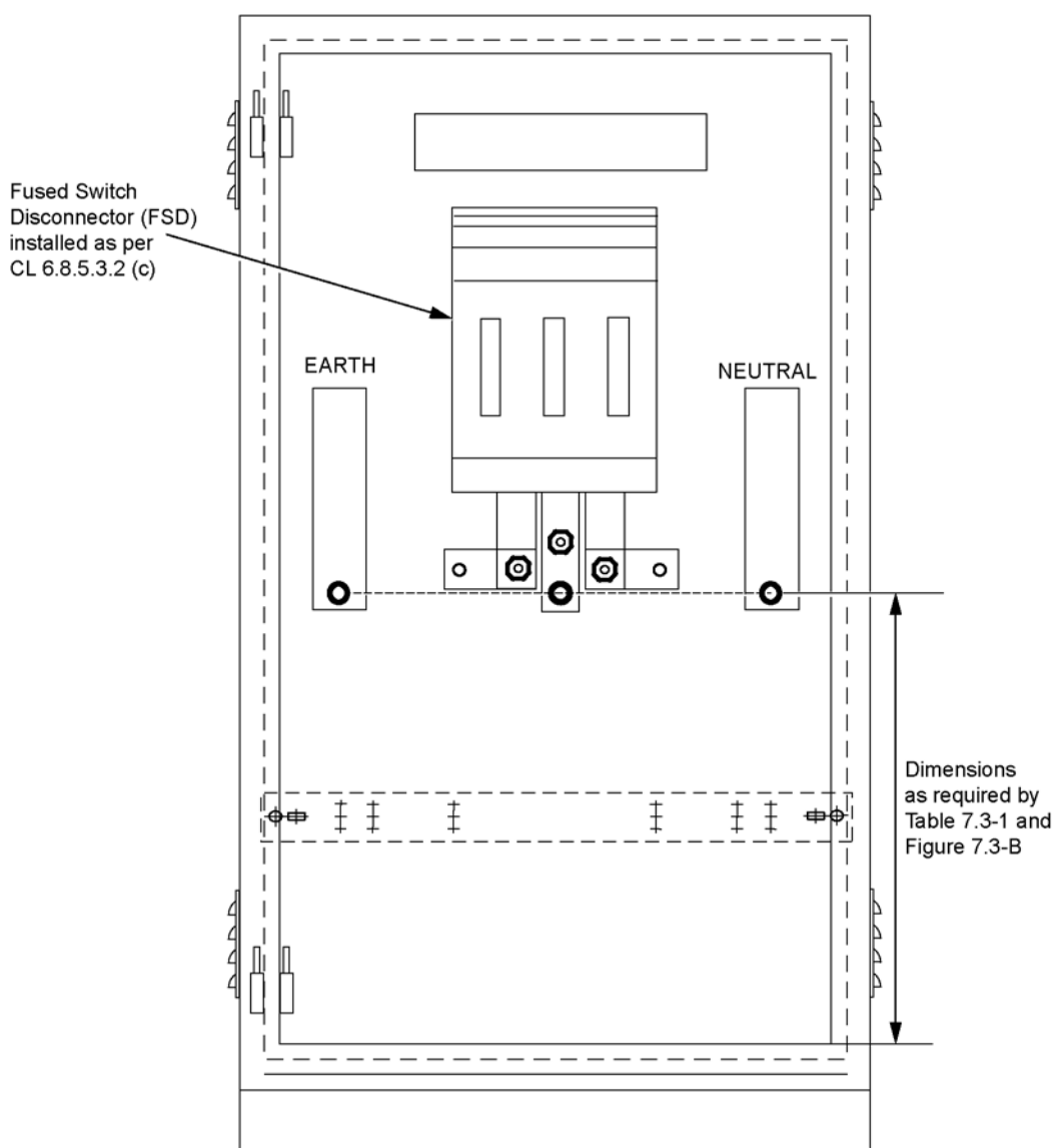
Figure 7.3-C Typical FSD Termination Method
