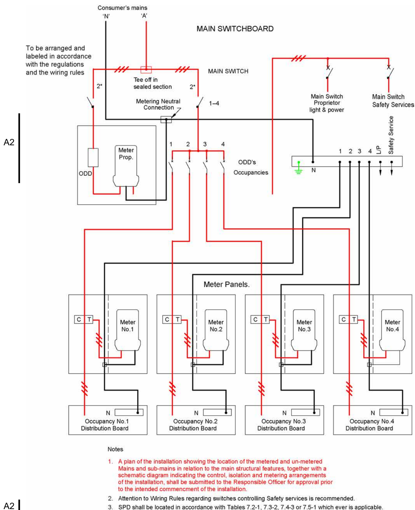
Figure 8.11-C Typical Wiring Diagram for 4 CT Metered Occupancies and Proprietor with Direct Connected Metering
