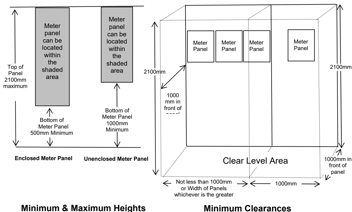
Figure 8.9-A Meter Panel Heights & Minimum Clearances
