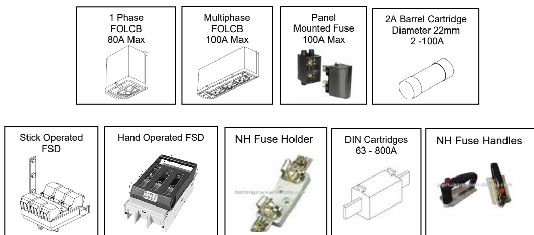
Figure 6.8-B Acceptable Supply Protection Devices and Assemblies
